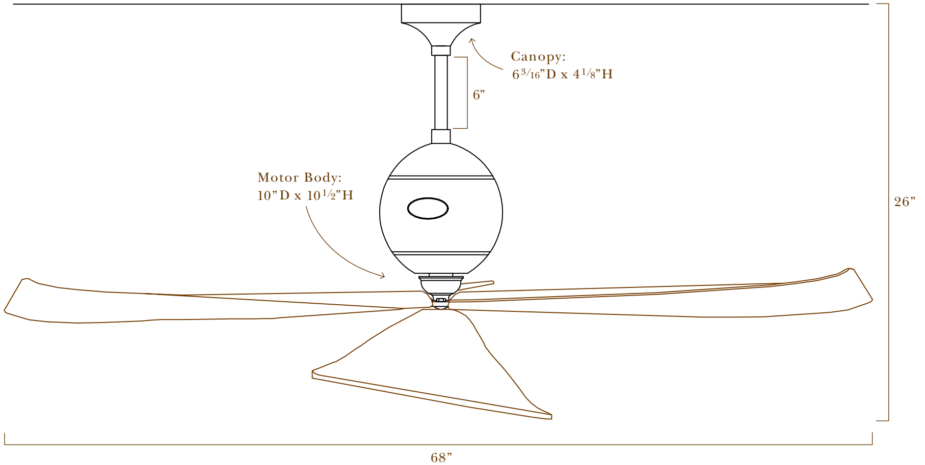
— THE ALISEO — Four Blade Ceiling Fan
